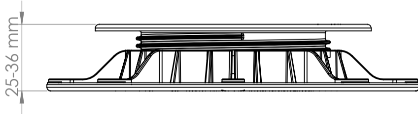
FRONT VIEW
