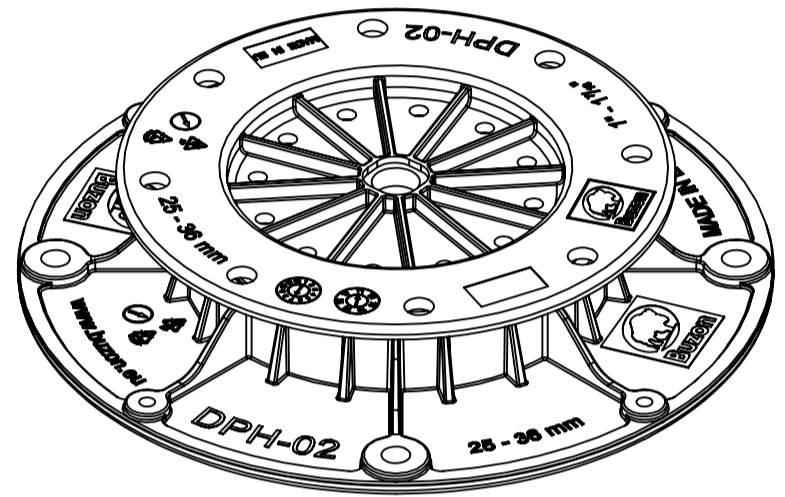
ISOMETRIC VIEW
