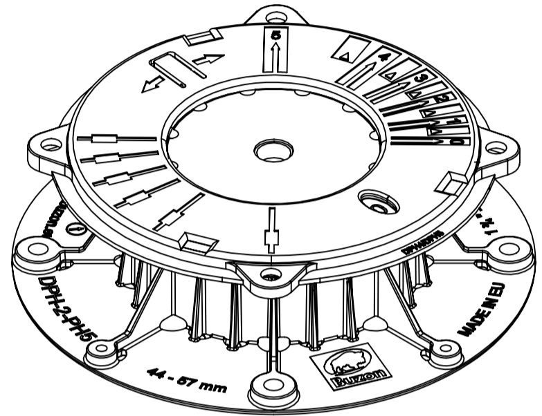
ISOMETRIC VIEW
