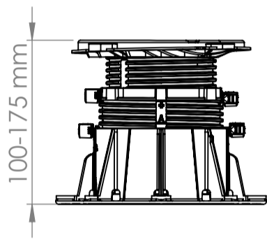
FRONT VIEW scale :1:5
