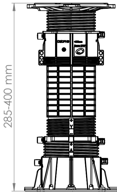
FRONT VIEW scale :1:5
