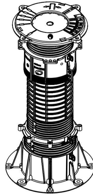
ISOMETRIC VIEW scale :1:5
