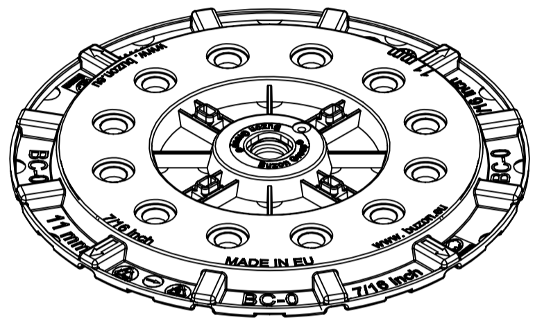
ISOMETRIC VIEW
