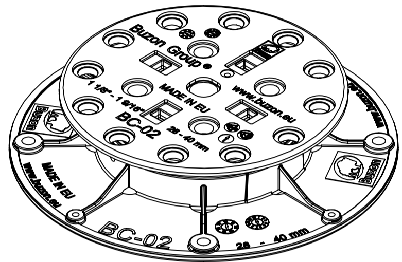
ISOMETRIC VIEW
