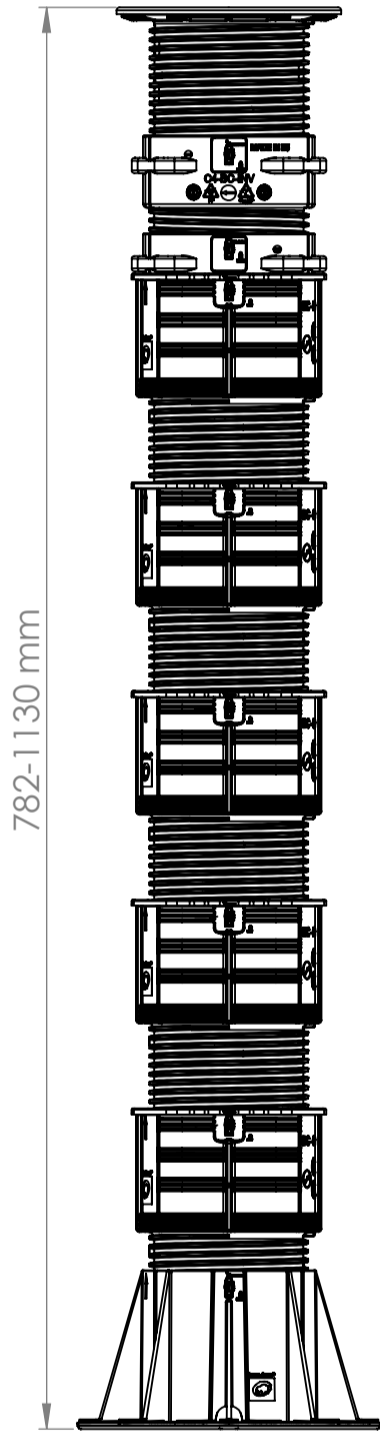
FRONT VIEW scale :1:5 ISOMETRIC VIEW scale :1:5
