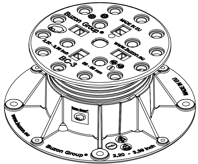
ISOMETRIC VIEW
