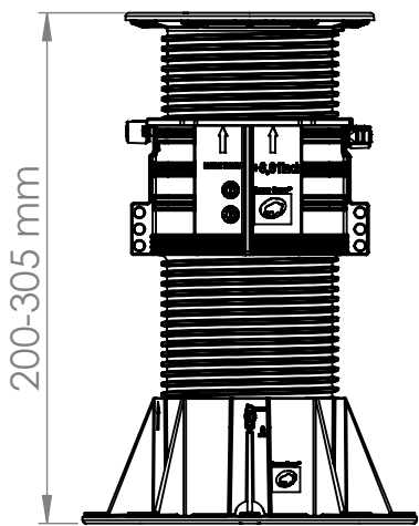
FRONT VIEW scale :1:5
