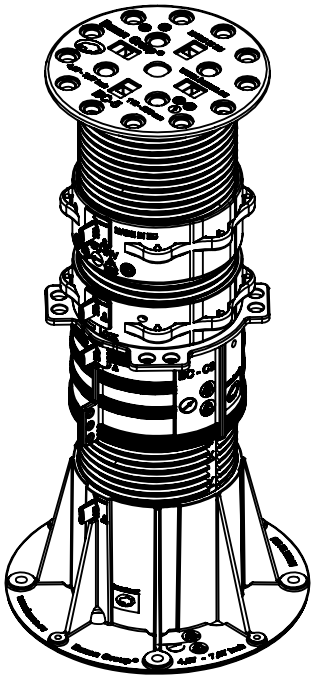
ISOMETRIC VIEW scale :1:5
