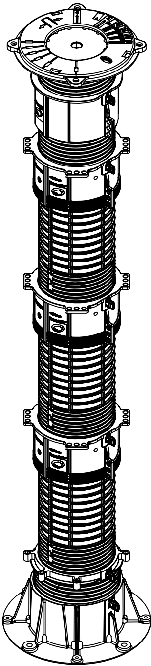
FRONT VIEW scale :1:5
