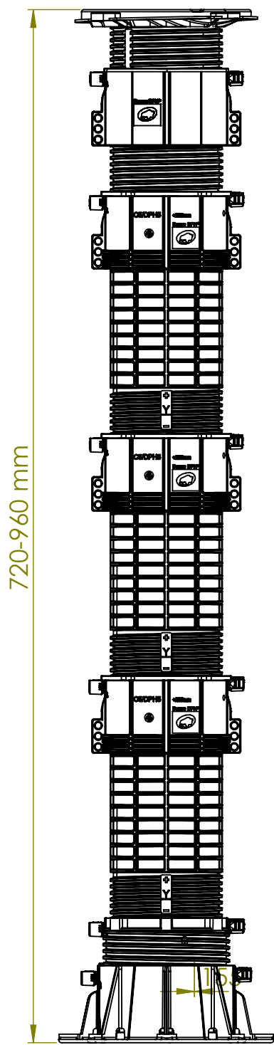
FRONT VIEW scale :1:5
