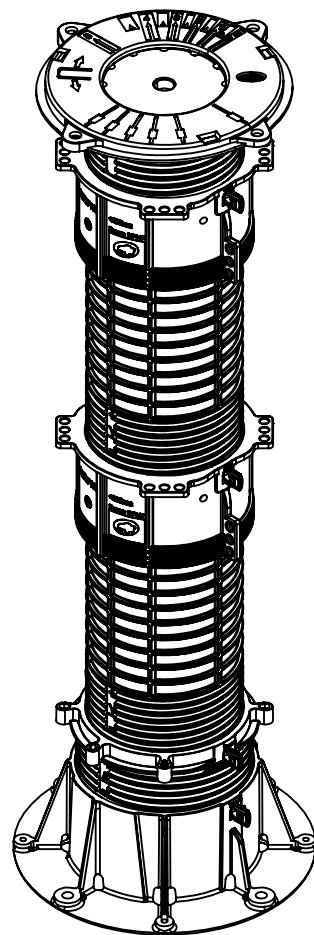
FRONT VIEW scale :1:5 ISOMETRIC VIEW scale :1:5
