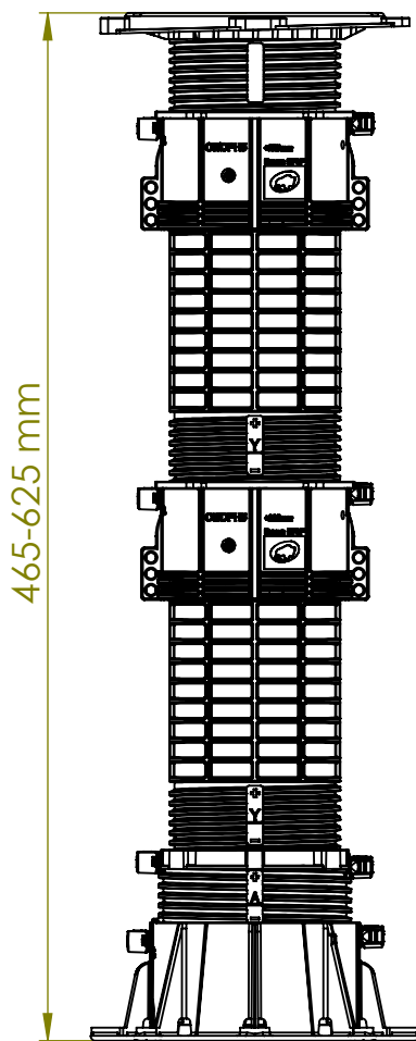
FRONT VIEW scale :1:5 ISOMETRIC VIEW scale :1:5
