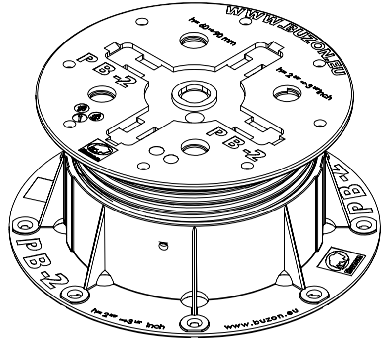
ISOMETRIC VIEW
