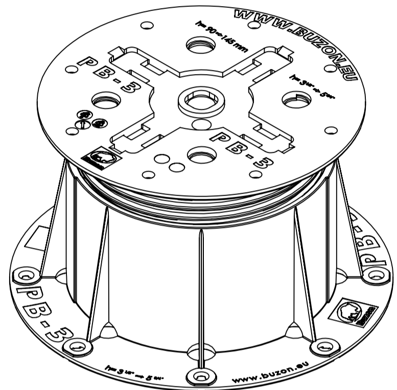
ISOMETRIC VIEW
