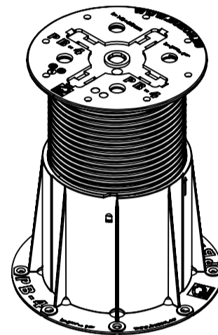
ISOMETRIC VIEW scale :1:5
