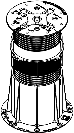
ISOMETRIC VIEW scale :1:5
