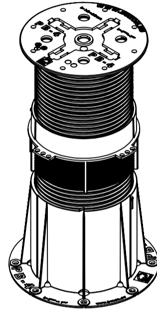
ISOMETRIC VIEW scale :1:5
