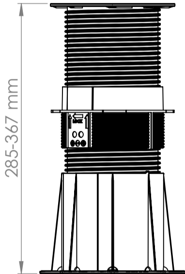
FRONT VIEW scale :1:5
